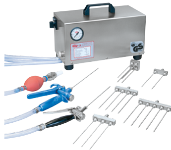
Inox Salt Injector
